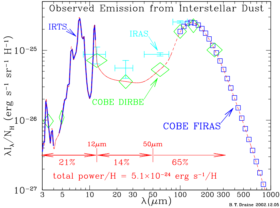
Figure 14: Observed emission from diffuse interstellar dust. Crosses: IRAS (Boulanger & Perault 1988); Squares: COBE-FIRAS (Finkbeiner et al. 1999); Diamonds: COBE-DIRBE (Arendt et al. 1998); Heavy Curve: IRTS (Onaka et al. 1996, Tanaka et al. 1996). The total power \sim 5.1 \times 10^{-24} \text{ erg s}^{-1}/\text{H} is estimated from the interpolated broken line.
