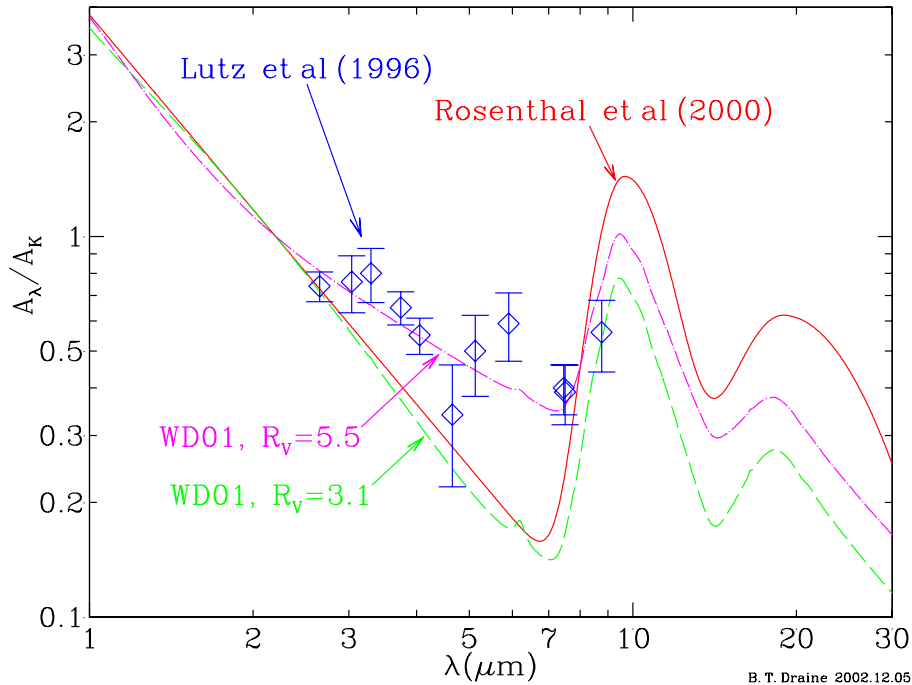
Figure 4: Infrared extinction, relative to extinction at K ( 2.2\ \mu\text{m} ), inferred by Rosenthal et al. (2000) for dust in the OMC-1 molecular cloud, and by Lutz et al. (1996) for dust toward Sgr A*, and as calculated for the Weingartner & Draine (2001a) grain models for R_V = 3.1 (60ppm C in PAH) and R_V = 5.5 (30ppm C in PAH). The 6.2\ \mu\text{m} absorption feature in the Weingartner & Draine (2001a) grain models is due to PAHs.
