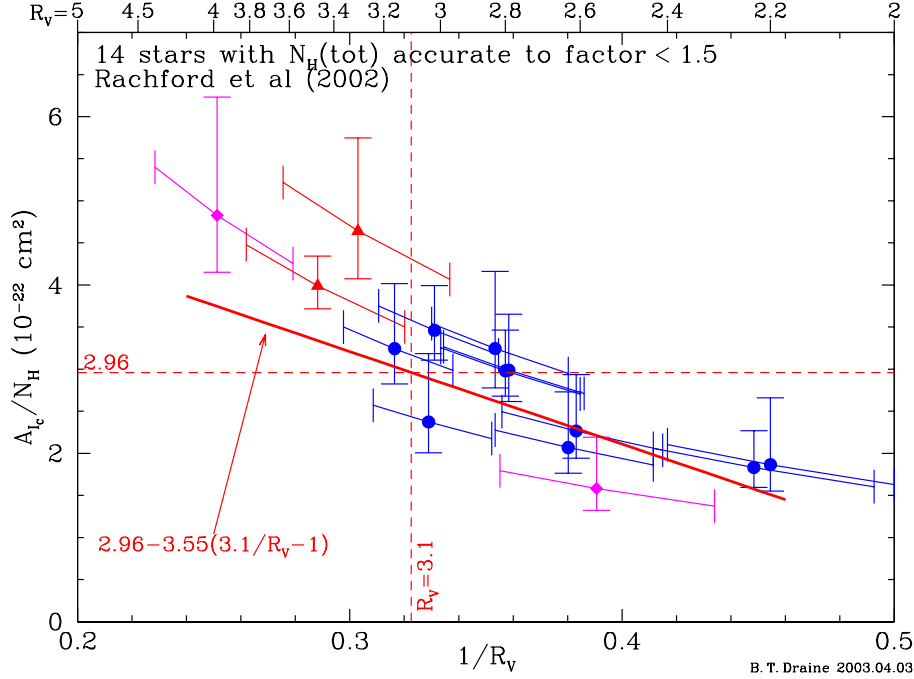
Figure 2: A_I/N_H for 14 sightlines through translucent clouds (Rachford et al. 2002), as a function of 1/R_V , with R_V determined by IR photometry (circles, R_V \pm 0.2 ); polarization \lambda_{\max} (triangles, R_V \pm 10\% ); or UV extinction curve (diamonds, R_V \pm 10\% ). Vertical error bars show 1\text{-}\sigma uncertainty due to errors in N_H ; tilted error bars show effects of errors in R_V . Least-squares fit [eq. 5] is shown.
