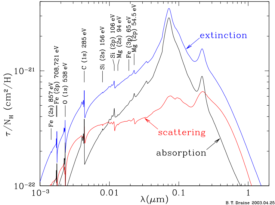
Figure 9: Extinction and scattering calculated for Weingartner & Draine (2001a) model for R_V = 3.1 Milky Way dust, but with abundances reduced by factor 0.93 (see text).
