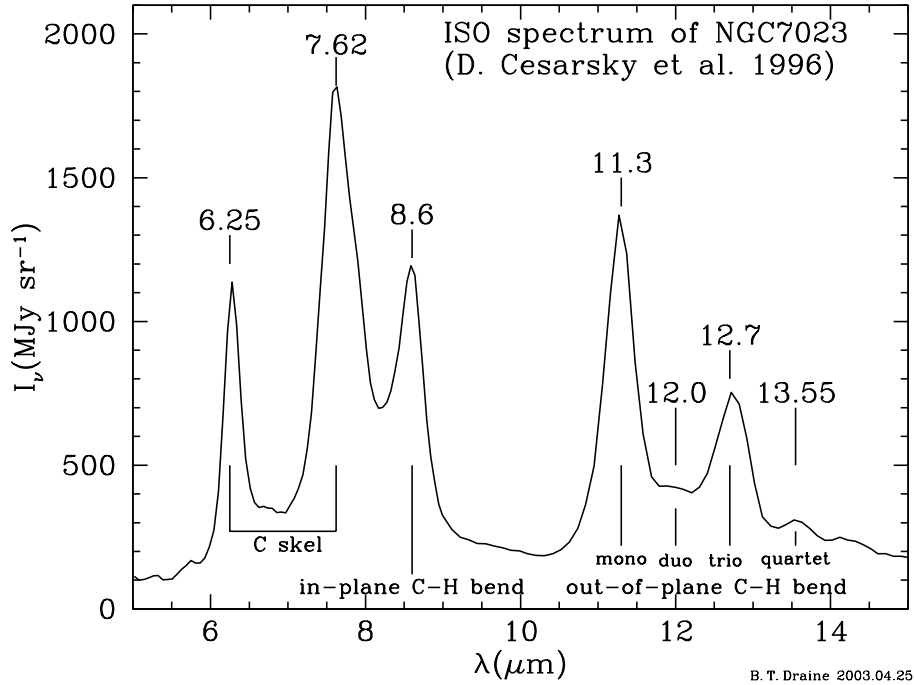
Figure 6: PAH emission features in the 5–15 \mu\text{m} spectrum of the reflection nebula NGC 7023.
