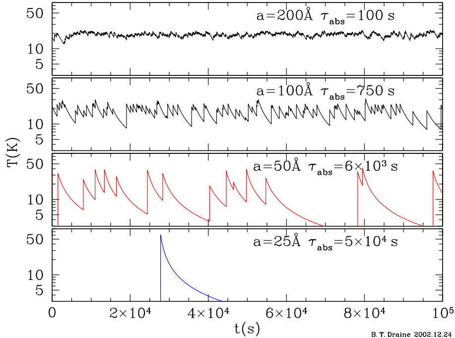
Figure 13: A day in the life of 4 carbonaceous grains, heated by the local interstellar radiation field. \tau_{\text{abs}} is the mean time between photon absorptions (Draine & Li 2001).
