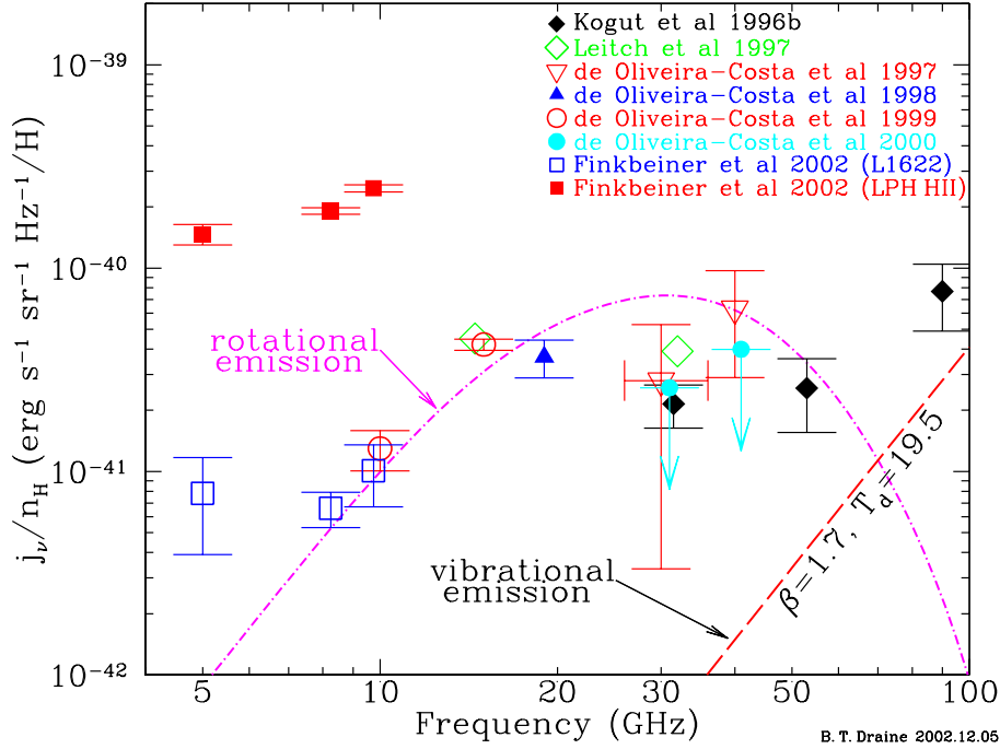
Figure 16: Dust-correlated microwave emission, expressed as microwave surface brightness per unit column density of hydrogen. Curves: theoretical estimate of Draine & Lazarian (1998a,b) . Symbols: observational determinations of “anomalous microwave emission”.
