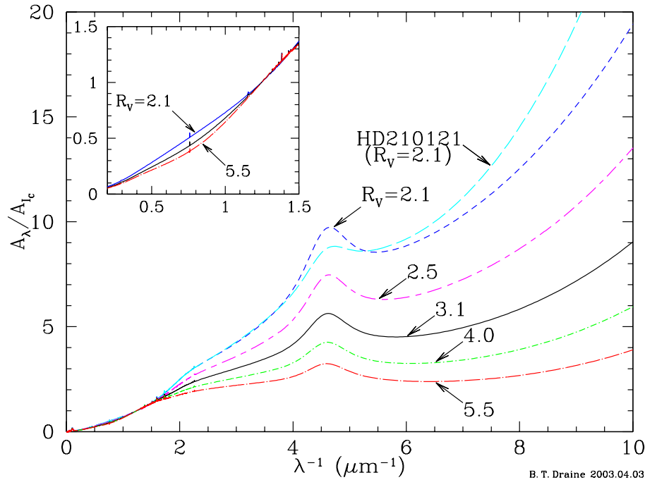
Figure 1: Extinction curves from prescription of Fitzpatrick (1999), with diffuse interstellar bands (DIBs) added as described in §3.3. The DIBs are barely visible on this plot.
