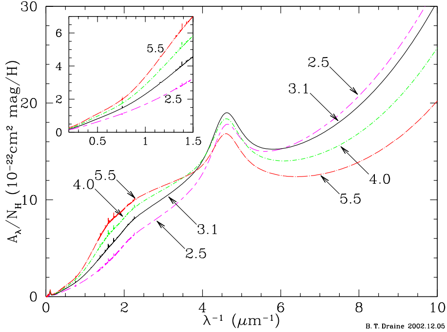
Figure 3: A_\lambda/N_H for different values of R_V , using F99 extinction curve fit and A_I/N_H from eq. (5).
