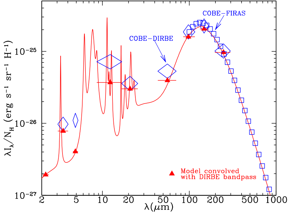
Figure 15: Solid line: infrared emission calculated for WD01 R_V = 3.1 Milky Way dust model (but with abundances reduced by factor 0.93) for grains heated by diffuse starlight (Li & Draine 2001b). Squares: COBE-FIRAS (Finkbeiner et al. 1999) Diamonds: COBE-DIRBE (Arendt et al. 1998).
