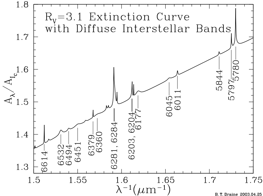
Figure 5: Diffuse interstellar bands in the 5700–6670Å region, using DIB parameters from Jenniskens & Desert (1994) .
