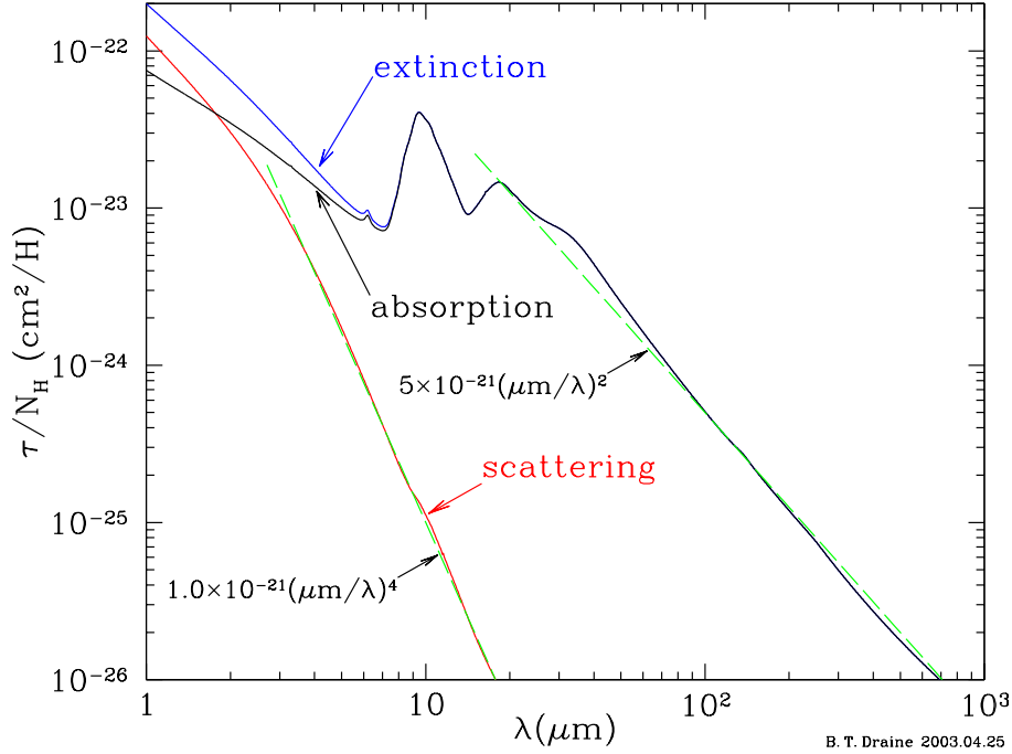
Figure 10: Extinction and scattering calculated for Weingartner & Draine (2001a) model for R_V = 3.1 Milky Way dust, but with abundances reduced by factor 0.93 (see text). The dashed lines show the asymptotic behavior of the absorption ( \propto \lambda^{-2} ) and scattering ( \propto \lambda^{-4} ) cross sections.
